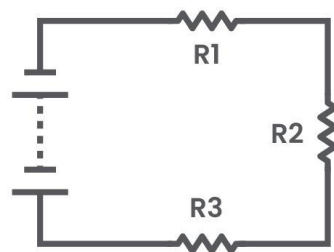
Series circuit
